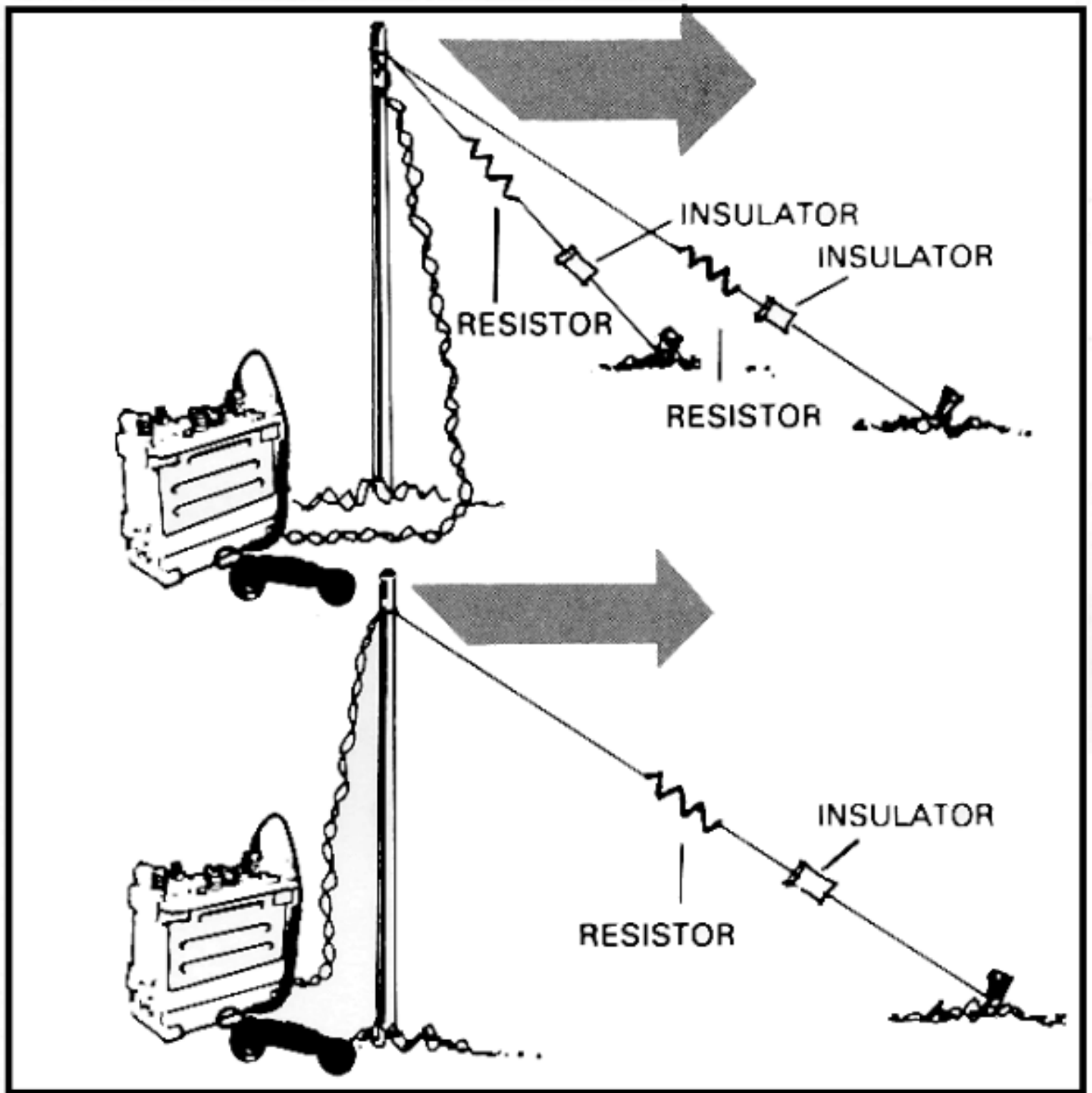
Figure 3-39. Sloping-V antenna.
