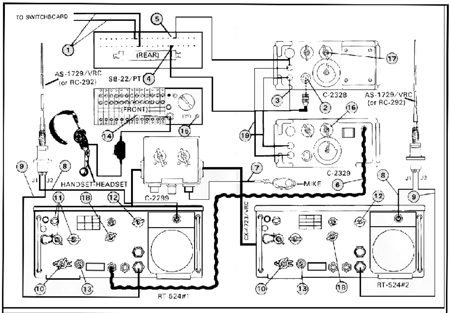
Figure F-15. NRI hookup using the AN/GR/ 35.
