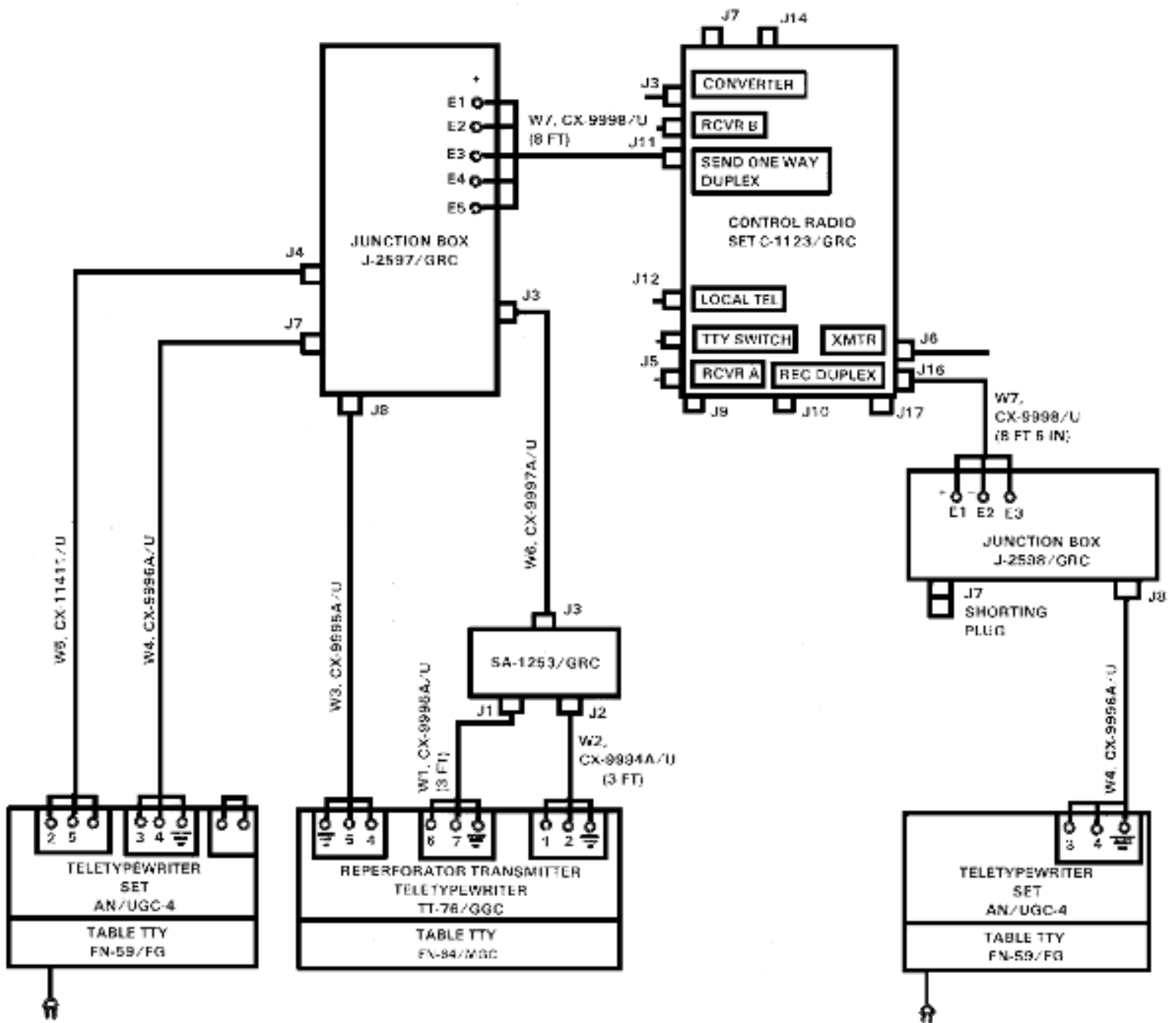
Figure 8-1. Wiring diagram for nonsecure operations, AN/GRC-26D.
